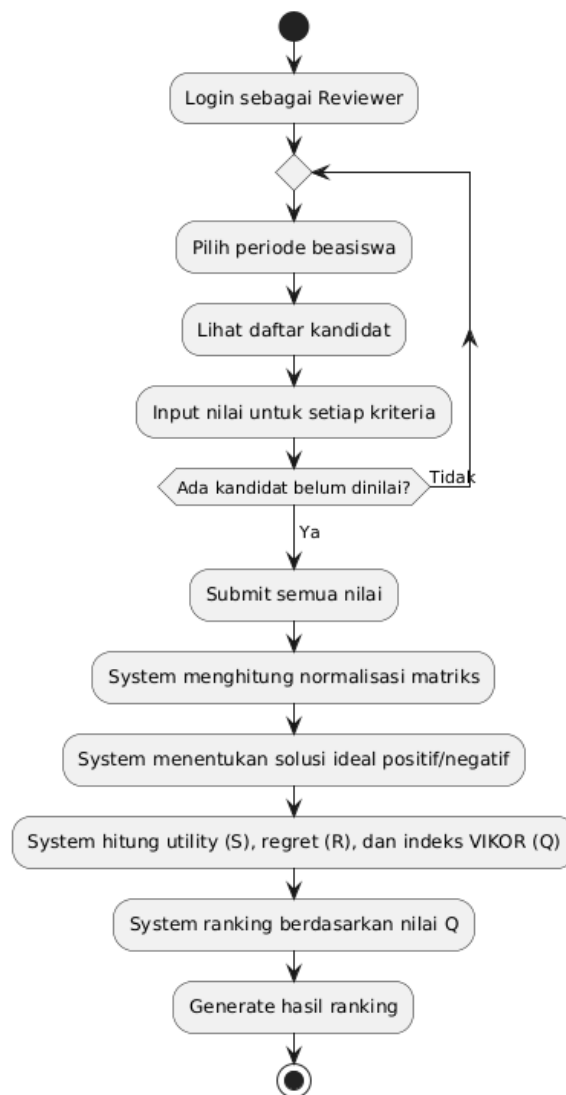
Gambar 2.3 Activity Diagram
