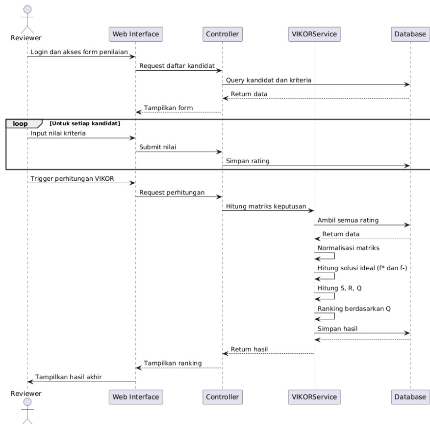
Gambar 2.4 Sequence Diagram
